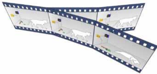
Figure 3 - Schrödinger's Cat
